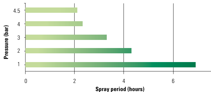
Spray period REB 15 AZ1 (Nozzle position mist)
