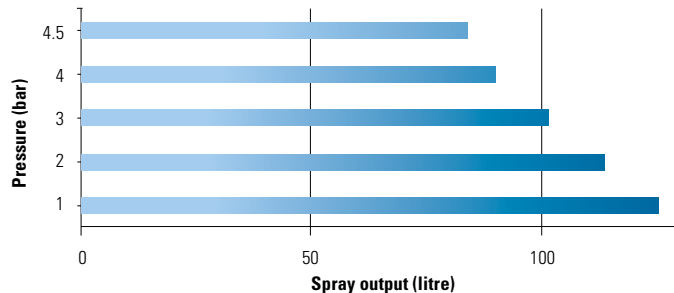
Spray output REB 15 AZ1 (Nozzle position stream)
